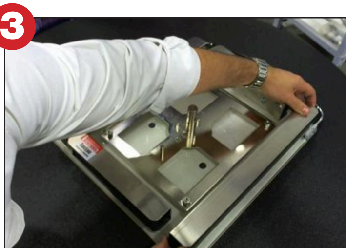
Step 3: Place the side 15" Gripper Channels just inside the Hoop Ring and down the side of the Adult Platen. Ensure the side Gripper Channels are installed approximately 1/4" from the edge of the platen.
