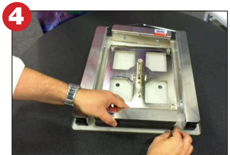
Step 4: Center the front and back 9" Gripper Channels between Side Gripper Channels. Ensure the front and back Gripper Channels are installed approximately 1/4" from the edge of the platen.
